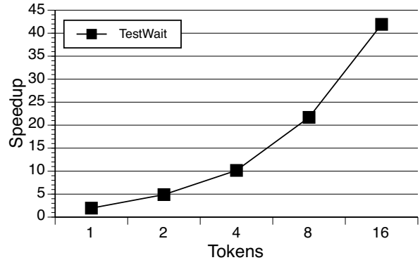
Figure 7. Speedup of token exchanges for TestWait with 32 processors, scaling the number of tokens from 1 to 16.
